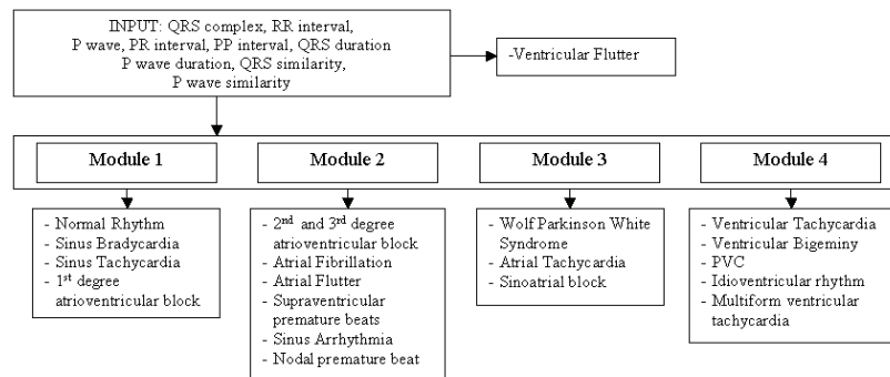
Figure 2: Decision tree like arrhythmia classifier.
