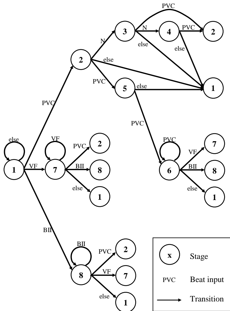
Figure 5: Deterministic automato used for arrhythmic episode detection and classification.
